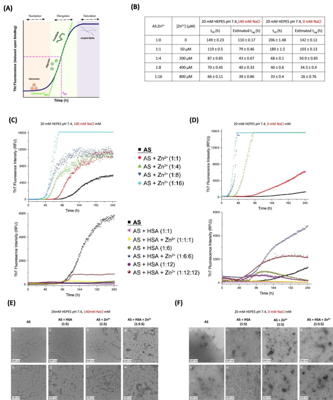
Fig. 1. Fibrillization kinetics of AS under pH 7.4, low and high ionic strength in the presence and absence of Zn 2+ and/or defatted human serum albumin (DE-HSA). (A) The nucleation dependent polymerization reaction of amyloid fibril formation causes a sigmoidal growth curve with nucleation, elongation, and saturation phases. (B) Table highlighting the estimated t 50 and t lag parameters for two experimental conditions setup. (C) AS fibrillization in the presence of increasing amount of Zn 2+ (AS:Zn 2+ , 1:1, 1:4, 1:8, 1:16 M ratio) and increasing amount of HSA and/or Zn 2+ under high-ionic strength (140 mM NaCl) and (D) under low-ionic strength (0 mM NaCl). (E) TEM images of fibrils formation of (a, b) AS (WT); (c, d) AS in the presence of HSA (1:5); (e, f) AS in the presence of Zn 2+ (1:5); (g, h) AS in the presence of HSA and Zn 2+ (1:5) under high-ionic strength and (F) under low-ionic (Scale bar: upper row 200 nm and lower row 100 nm). Credit: International Journal of Biological Macromolecules (2022). DOI: 10.1016/j.ijbiomac.2022.10.066
