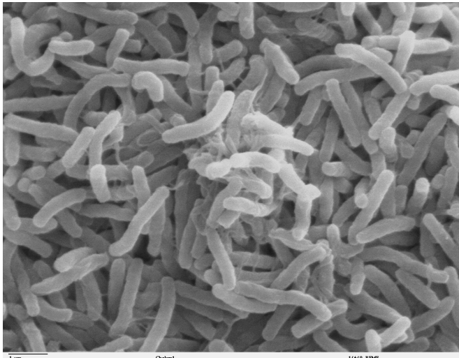
Scanning electron microscope image of V. cholerae . Credit: public domain
