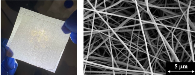
Left: A nanofiber filter that captures 99.9% of coronavirus aerosols; Right: A highly magnified image of the polymer nanofibers. Credit: Yun Shen
