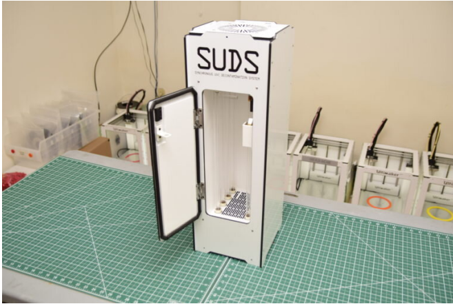
Synchronous UV Decontamination System, or SUDS. Credit: Case Western Reserve University
