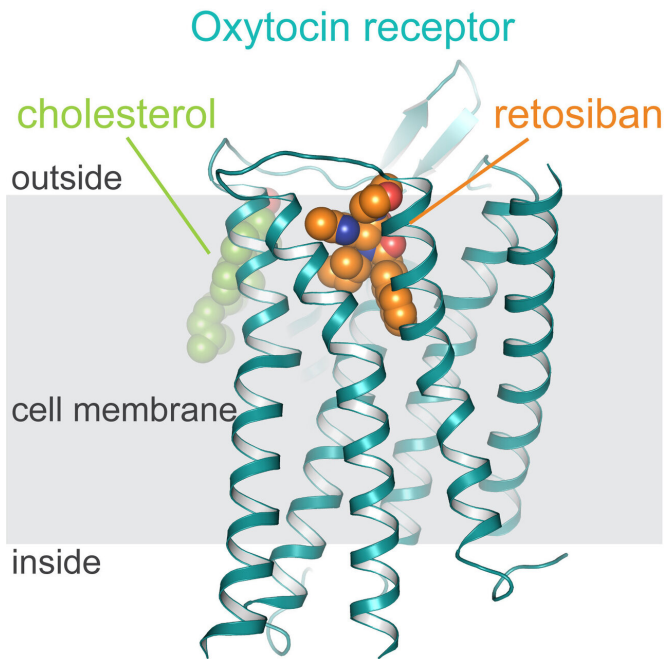
Structure of the oxytocin receptor in the cell membrane (grey), to which retosiban (orange) and cholesterol (green) are bound. Credit: University of Zurich
