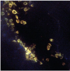
Neuron
