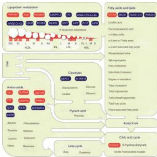
Overall summary of basic metabolism, key constituents of the serum metabolome and associated genetic regions. [doi:10.1038/ng.10730]
